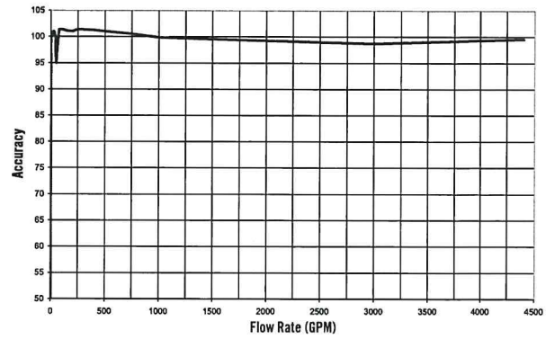
Accuracy – 8" with 2" PD Bypass
