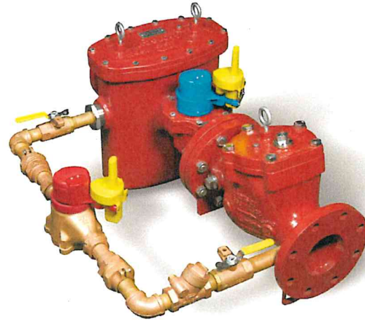
4" x 1" FM 3 with Residential Fire Meter
