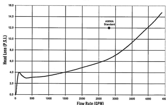
Head Loss – 8" with 2" PD Bypass
