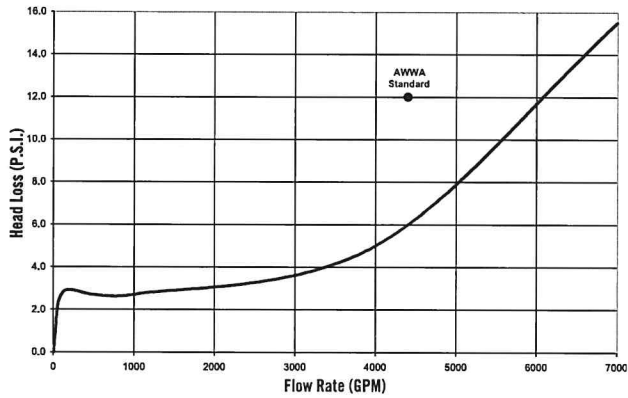
Head Loss – 10 with 2" PD Bypass Meter
