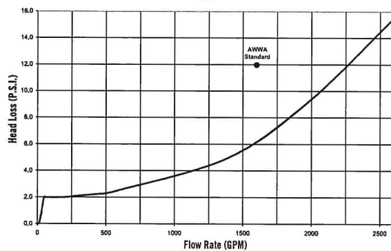
Head Loss – 6" with 2" PD Bypass
